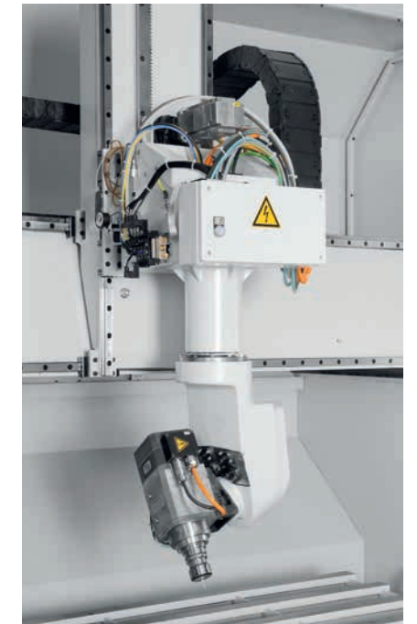
Cardanic 5-axis working head of the ECO-LT with an undercut of up to 46°.
