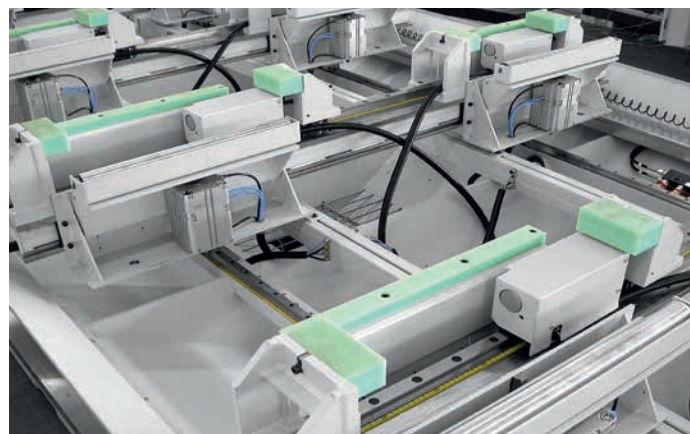
Pneumatic horizontal clamping devices in heavy design with support rollers.
