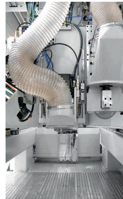
Working unit with automatic tool change for vertical milling, drilling, sawing and grinding work, supplemented by a sawing unit on a separate positioning slide.
