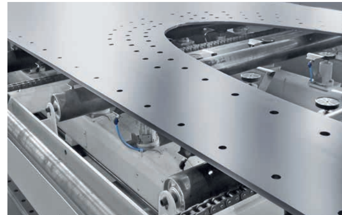
Tower section of a wind power unit on a pin table with rollers and transverse conveyor.
