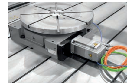
NC-rotary table for precision rotary milling components (for example an aircraft turbine ring).
